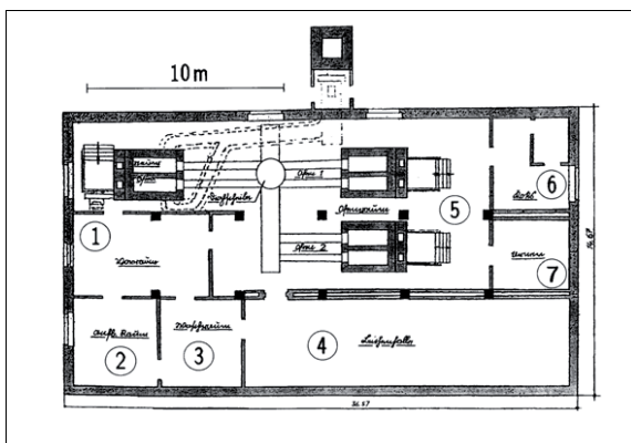
Illustration 1: Floor plan of crematorium 1 in Main Camp Auschwitz I in its original design. Allegedly the mortuary was later used as a ‘gas chamber’. 1: vestibule; 2: morgue; 3: wash-room; 4: mortuary (‘gas chamber’); 5: furnace room; 6: coke storage room; 7: urn room.
