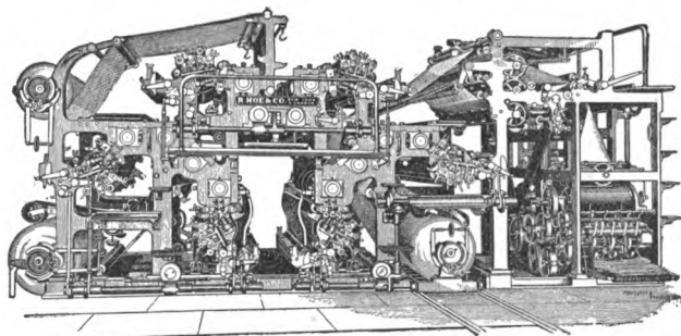
THE HOE SEXTUPLE STEREO TYPE PERFECTING PRESS AND FOLDER. Prints 72,000 4, 6, or 8-page papers per hour; 48,000 10 or 12-page papers per hour; 36,000 16-page papers per hour; 24,000 14, 20, or 24-page papers per hour; all the dimensions of the average daily newspaper, and delivered folded and counted.
