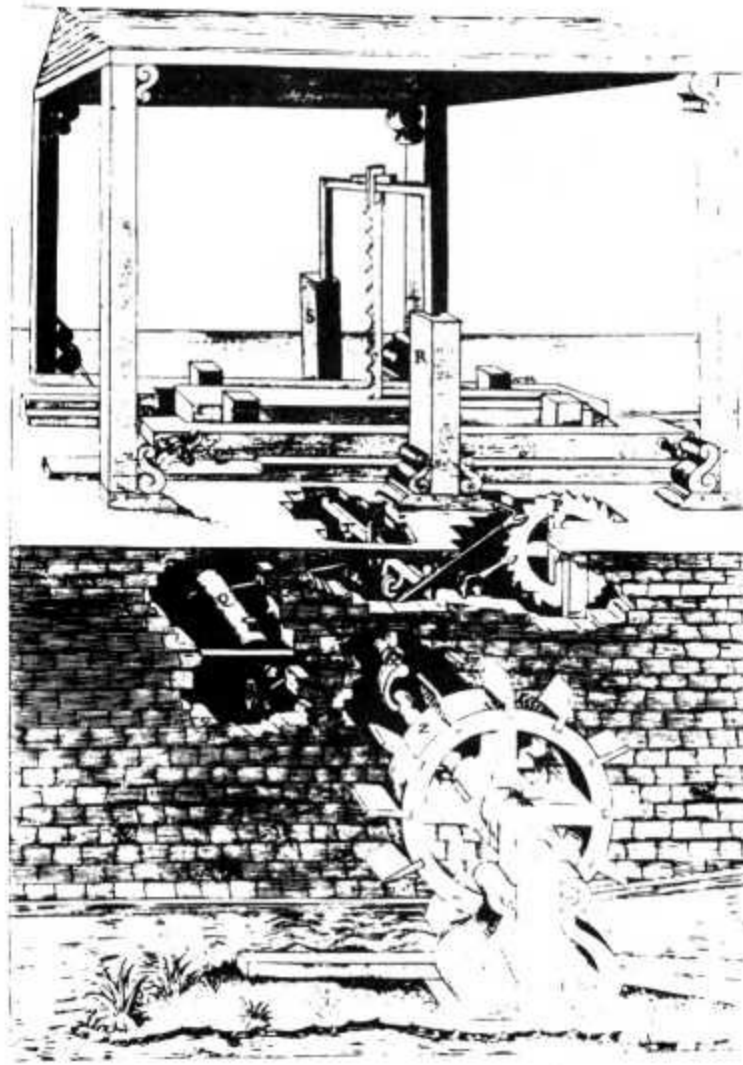
Figure 16. Water-driven sawmill as depicted by Ramelli in 1588.
