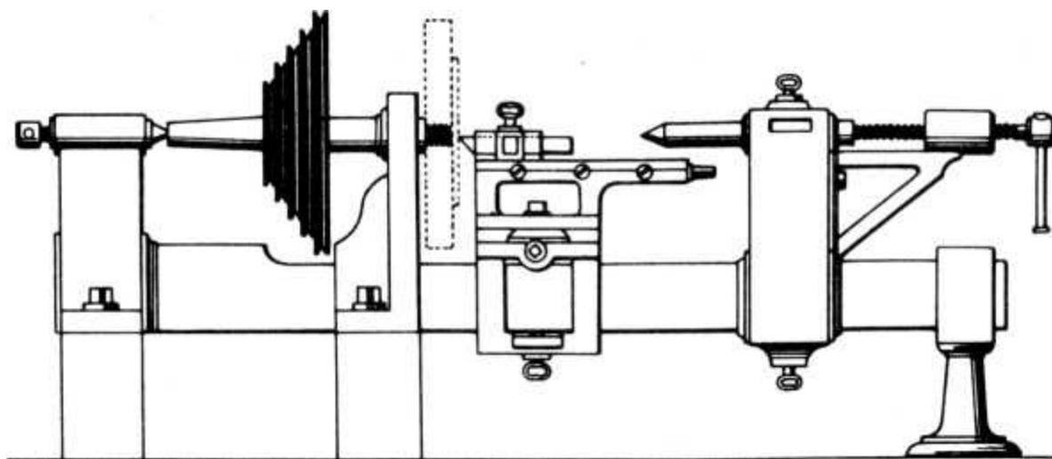
Figure 31. Henry Maudslay's slide and finishing lathe, dating from 1800. Source: Maurice Daurnas, A History of Technology and Invention , Vol. III, Crown Publishers Inc., New York.
