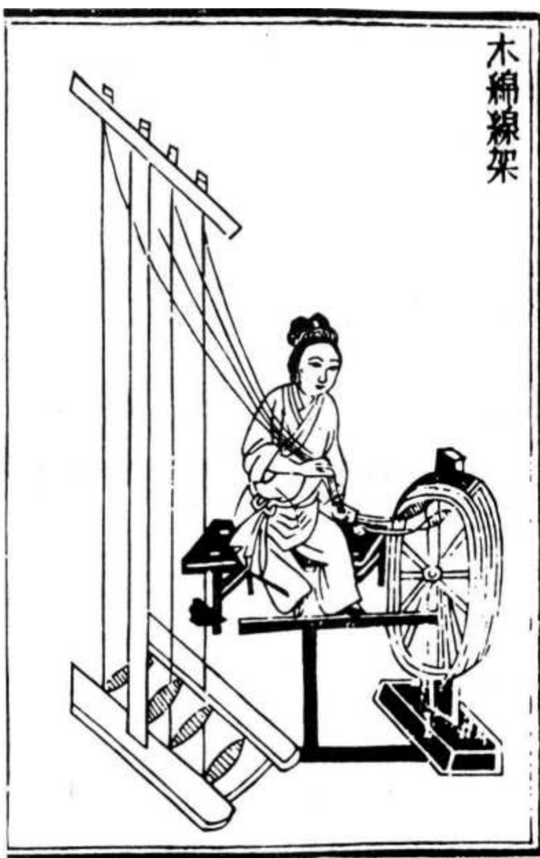
Figure 44. Spindle wheel for doubling (twisting together two separate yarns). The wheel is operated by it treadle.
