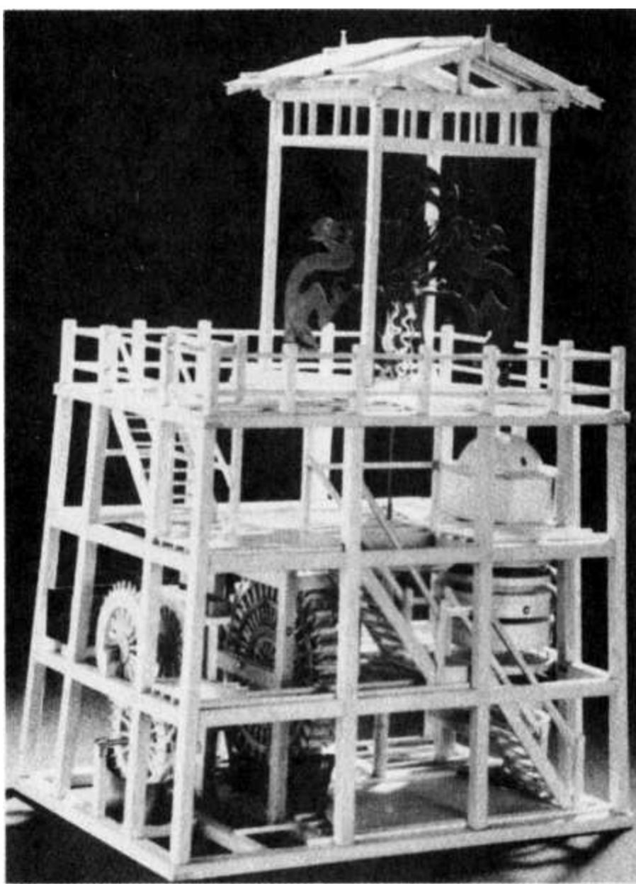
Figure 46. Model of the "Great Cosmic Engine" made by Su Sung ill 1086. The clock had it mechanical escapement, but was turned by water power.
