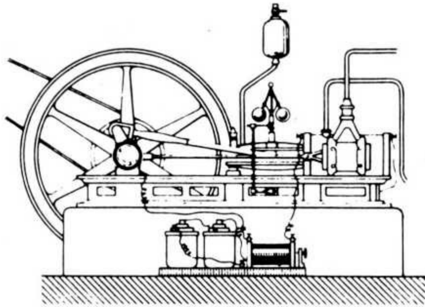
Figure 36. Gas engine, built by Lenoir in 1860.
