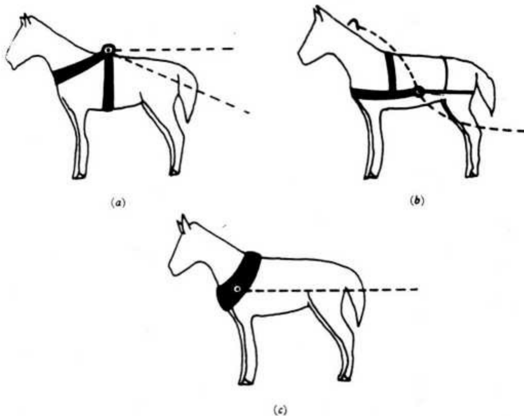
Figure 7. Three forms of horse harness: (a) depicts the inefficient throat-and-girdle harness used in antiquity; (b) shows the breast strap employed in the early middle ages; (c) shows the shoulder collar introduced in the later middle ages.
