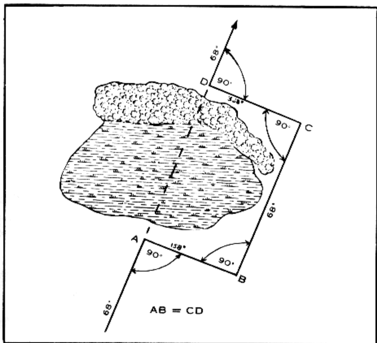
Figure 38. 90^\circ method of offset.
