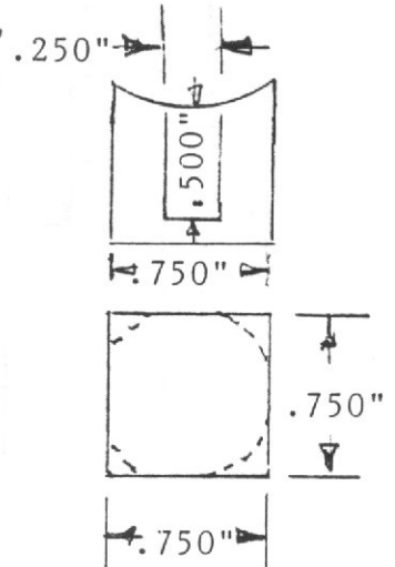
Front Hinge Block. Weld in place.
