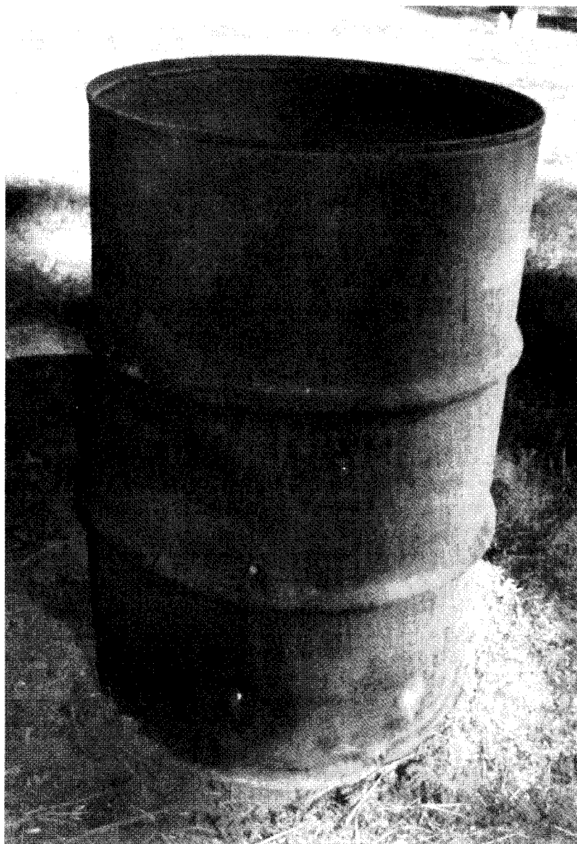
A 55-gallon steel burn barrel for disposal of soiled waste and other burnable trash. Note the vent holes.
