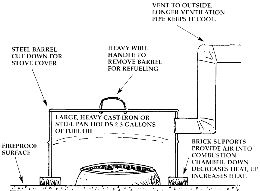
Homemade spark-type oil heater. A very low blue surface flame burns fumes from oil, heating the room. Refill once per day from portable can.
