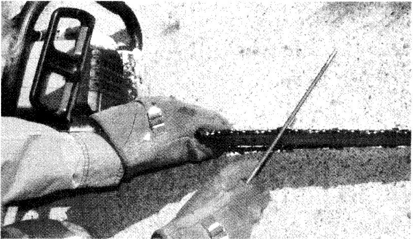
Chain saw chain teeth must be filed one direction toward the outside.
