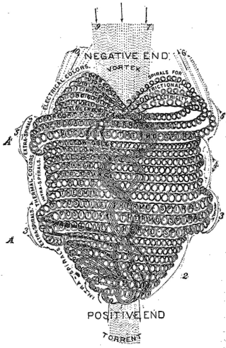
Fig. 135. The general Form of an Atom, including the spirals and 1st Spirillae, together with influx and efflux ethers, represented by dots, which pass through these spirillae. The 2nd and 3rd spirillae with their still finer ethers are not shown.
