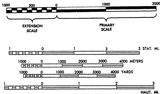
Figure 5-19.—Graphic scale.
