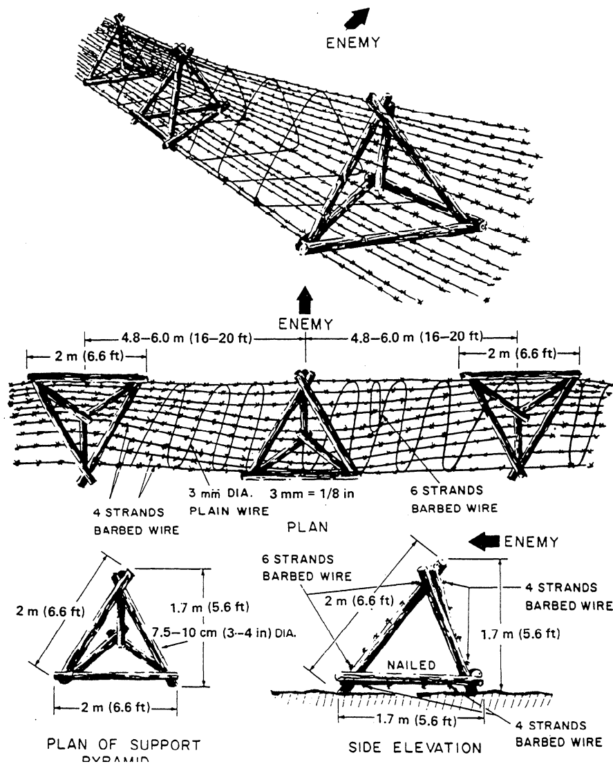
Figure 8-32.—Lapland fence.
