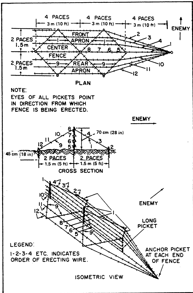
Figure 8-20.—Double-apron fence.
