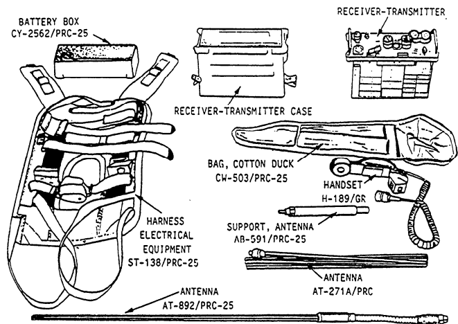
Figure 11-1.—Radio Set AN/PRC-77 components.
