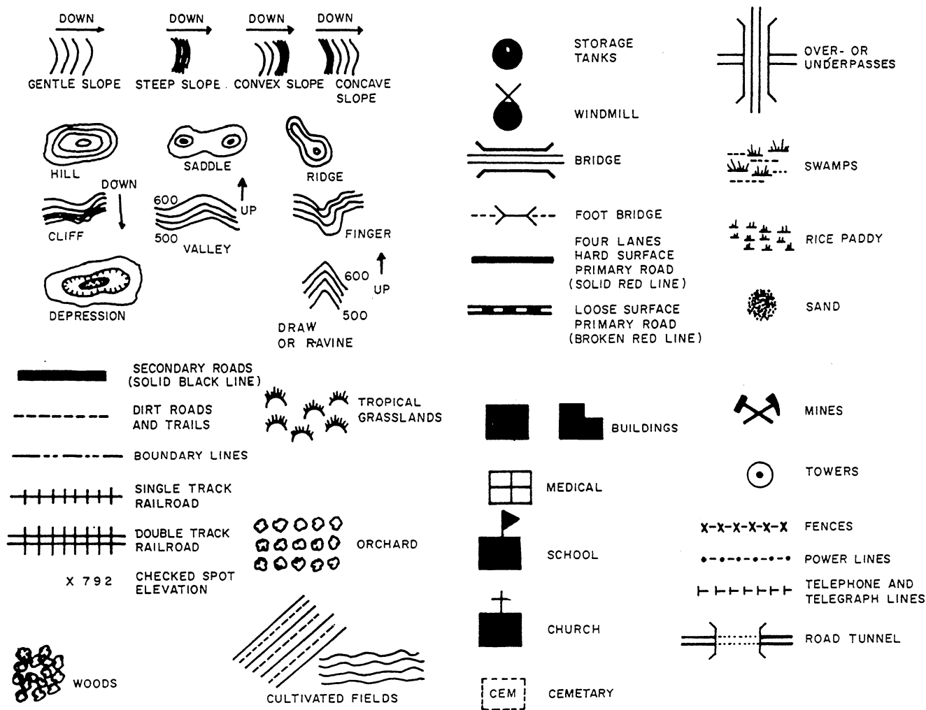
Figure 5-22.—Topographic symbols.
