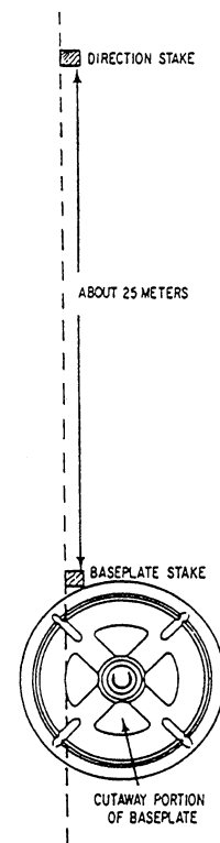
Figure 14-12.—Placing baseplate against baseplate stake.
