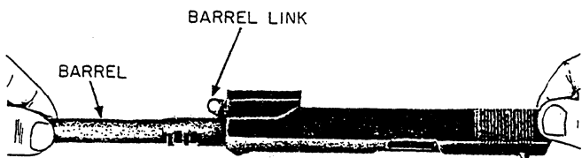
Figure 3-36.—Barrel removal from the slide.
