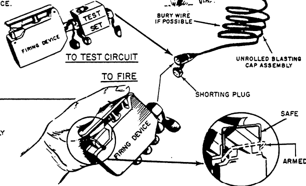
Figure 12-17.—The instruction sheet attached to the M7 bandoleer.
